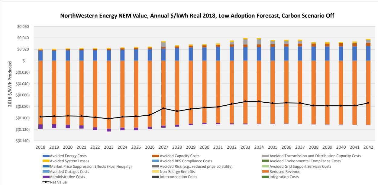
Figure 10. Annual Net Value in Real $/kWh Based on RIM Test, Low Adoption, Carbon Off
