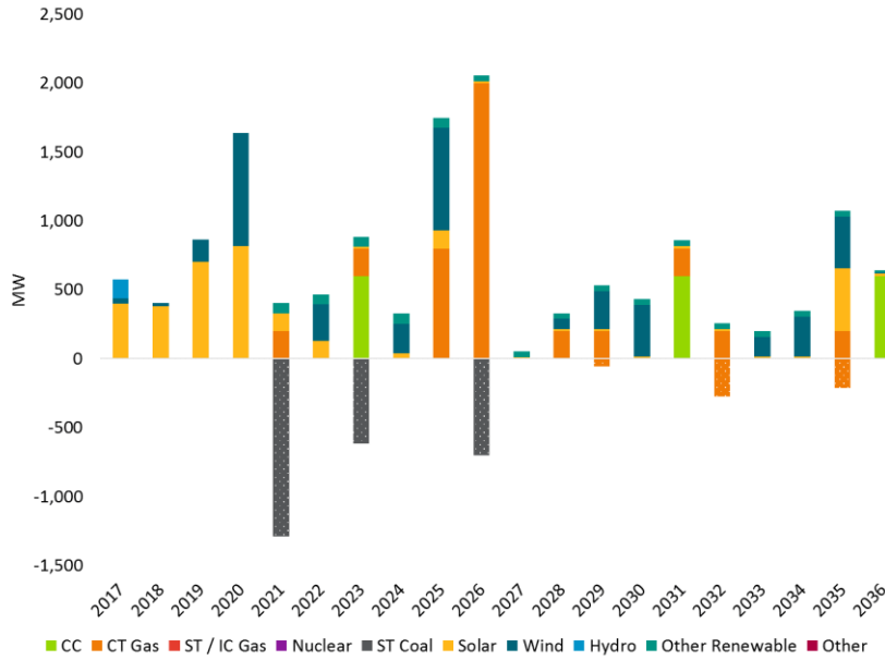
Figure 7. Capacity Additions and Retirements
