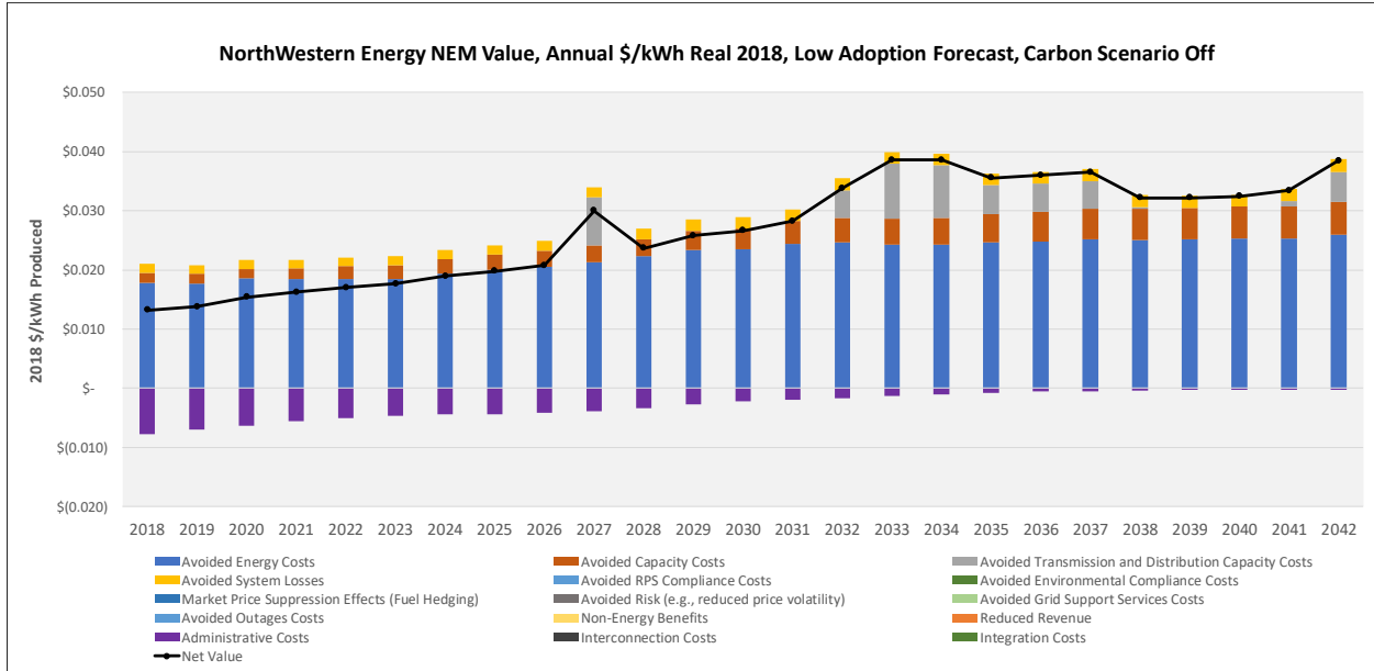
Figure 9. Annual Net Value in Real $/kWh Based on UCT Test, Low Adoption, Carbon Off
