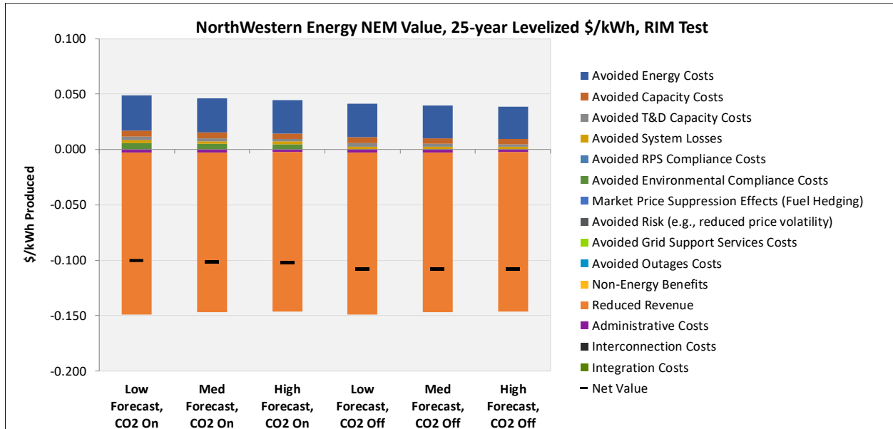
Figure 4. Graphical Levelized Net Avoided Costs Based on RIM Test
